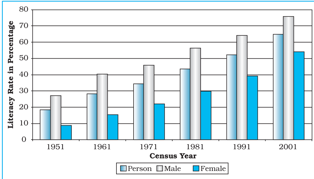
Fig. 3.6 : Literacy Rate, 1951-2001
