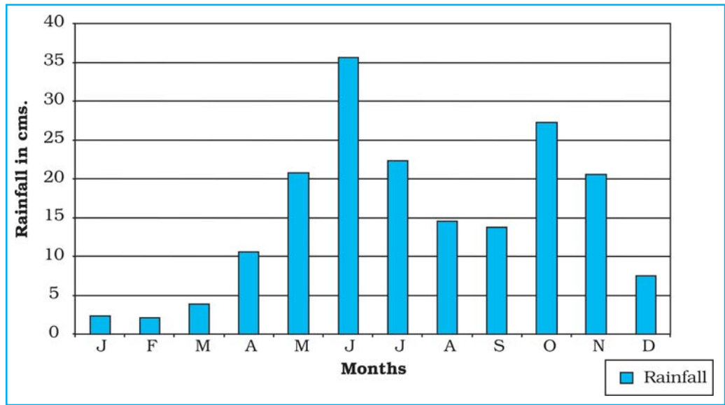
Fig. 3.4 : Average Monthly Rainfall of Tiruvanantapuram
