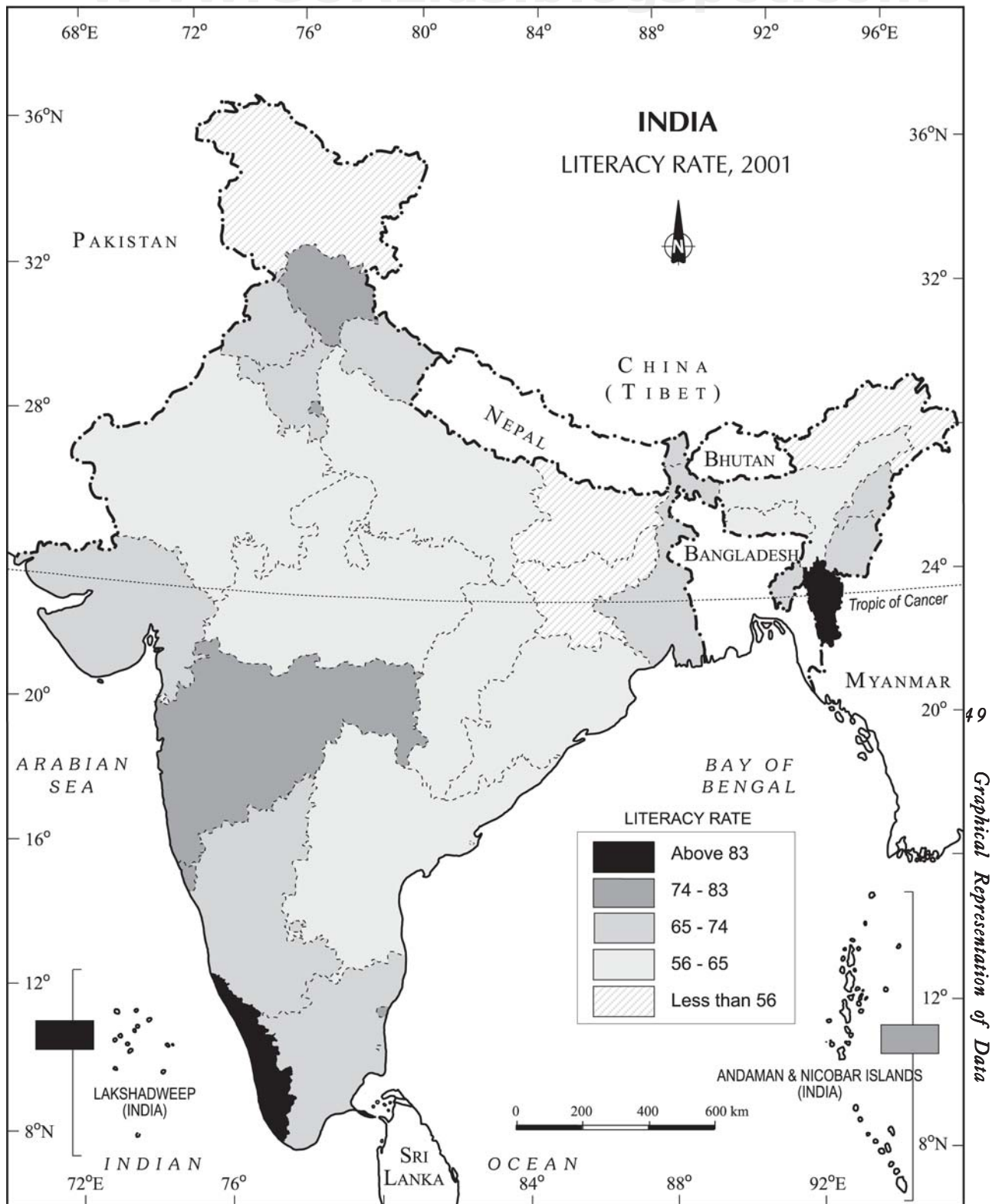
Fig. 3.14 : Literacy Rate, 2001
